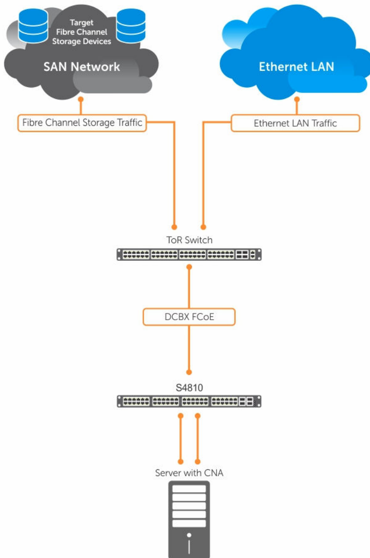
Figure 34. FIP Snooping on a Switch
